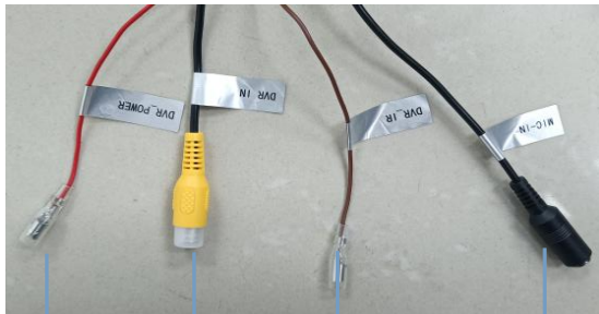
12V VBS_DVR DVR_IR External microphone
