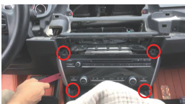
10. Remove the fixed screws, and take out the panel.
