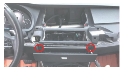
6. Remove the fixed screws and take out the storage box.
